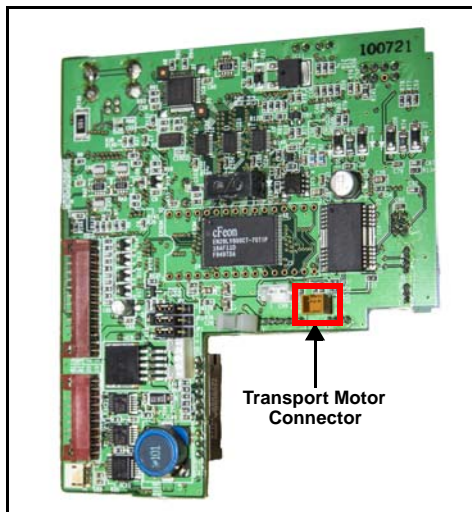
Figure 1: UBA IL-S Series CPU Board
