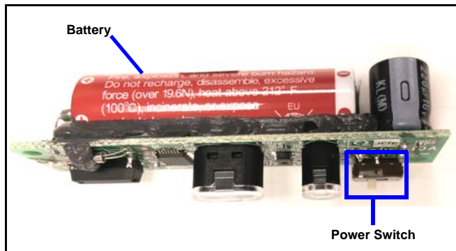
Figure 1: UBA® ICB® PCB Module (Standard Cash Box)
