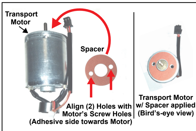
Figure 1 UBA® Transport Motor and Motor Spacer
