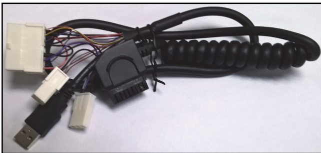
Figure 1 GEN5™/GEN2U™ Coil Harness w/ Secondary RS-232 Connector
